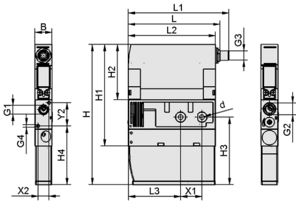
Design data SCPi 20 NO VD M12-5
