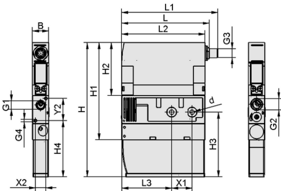
Design data SMPi 20 NC VD M12-5
