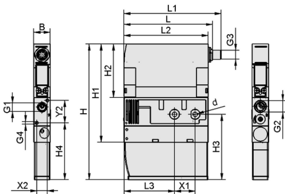
Design data SCPi 15 NC VD M12-5
