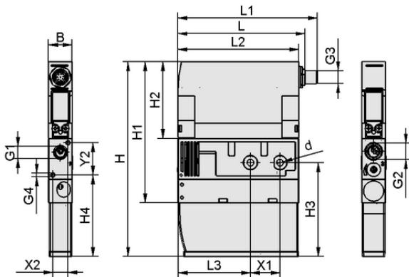
Design data SMPi 15 NC VD M12-5
