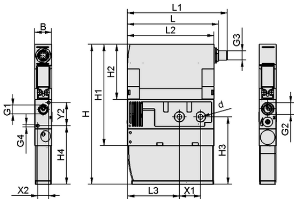
Design data SMPi 15 NO VD M12-5
