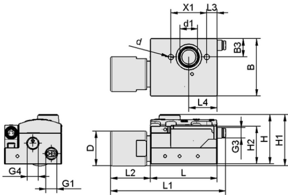
Design data SEAC 10 RP R
