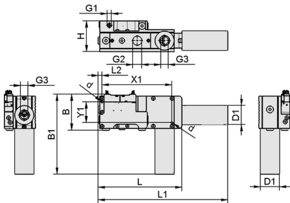
Design data SEM-C 25 SDA NO AS
