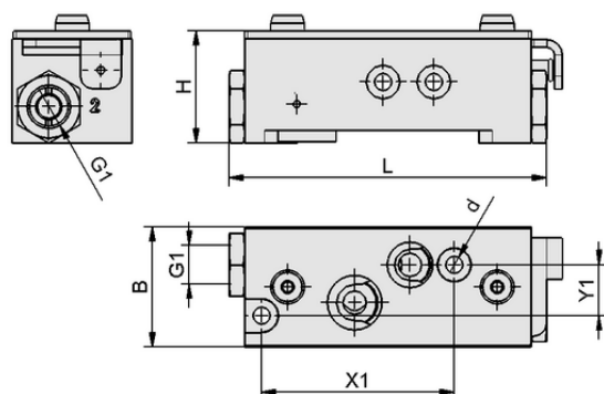
Design data GPQ1 122x46x43 SXPi/SXMPi
