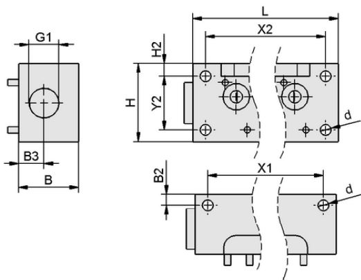
Design data GP 2 SMP 15..30/SCP 20..30
