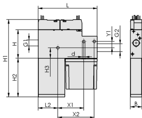
Design data SCP 30 NO AS
