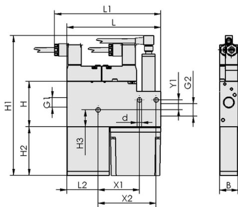
Design data SMP 25 NO AS RD
