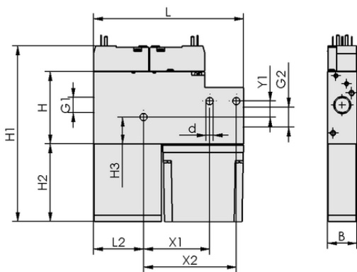
Design data SMP 25 NO AS
