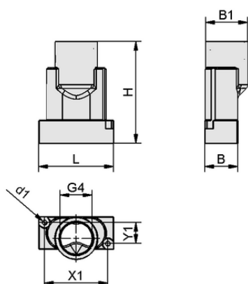
Design data ABL-SET SBPL/SCPL L
