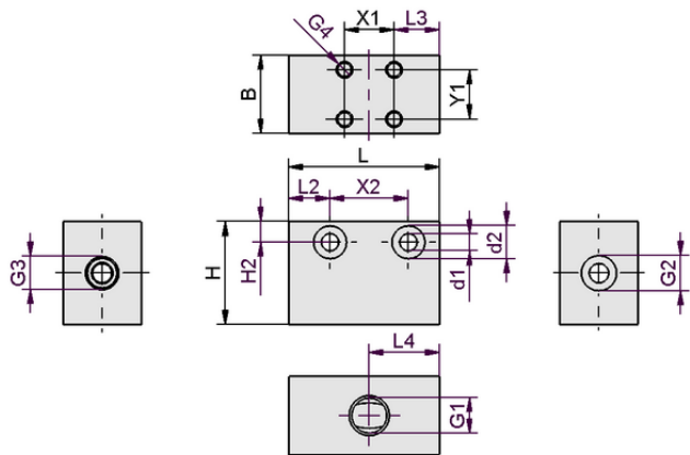
Design data SFE 13 POM
