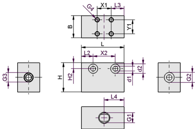
Design data SFE 22 POM
