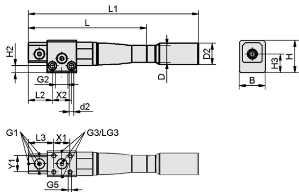
Design data SBP HV 2 16 22 S SD
