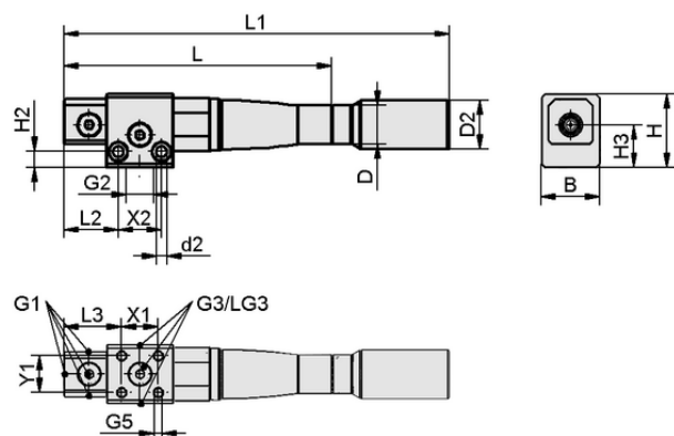
Design data SBP HF 3 06 13 SD
