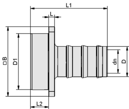
Design data ST 25 AL-EL
