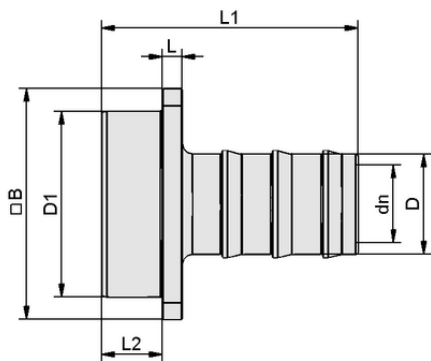
Design data ST 20 AL-EL
