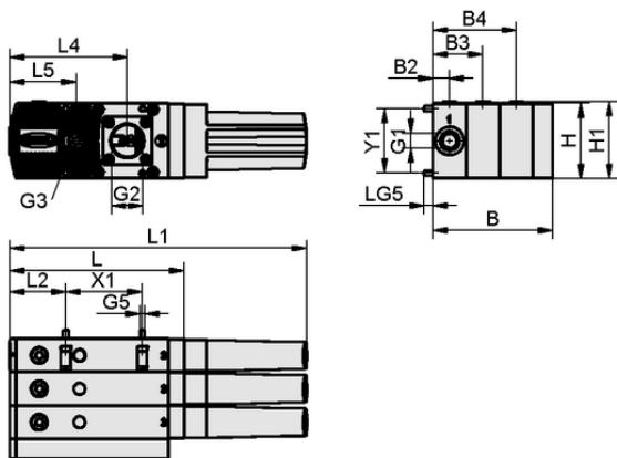
Design data SBPL 150 HF
