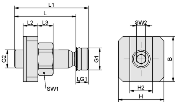
Design data SET SFE 13
