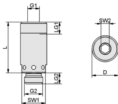
Design data SEV G1/8-IG G1/4-AG
