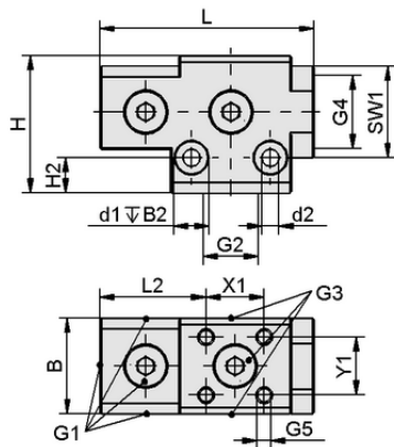
Design data SFE 22 AL
