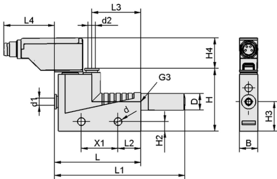
Design data SBP-C 25 S03 VS-T
