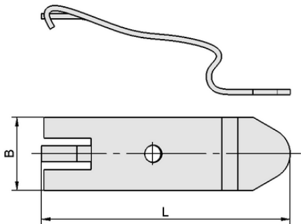
Design data SET SBP M4-IG
