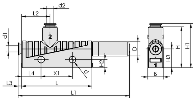
Design data SBP 25 S03 SDA
