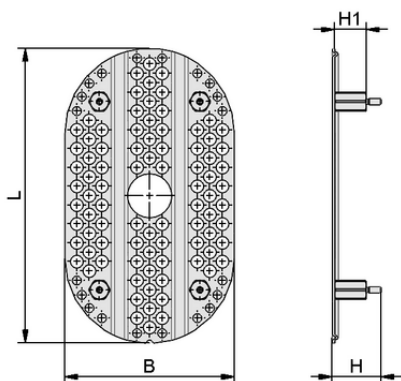
Design data LOCH-PL 235x135x39 ST PSSG
