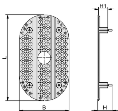
Design data LOCH-PL 202x127x29 ST PSSG
