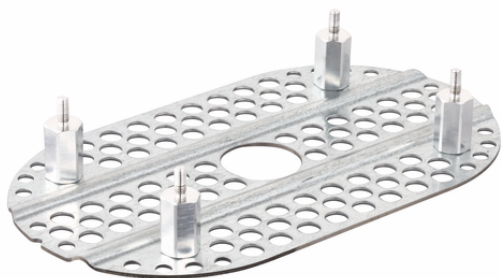
LOCH-PL 288x188x44 ST PSSG
