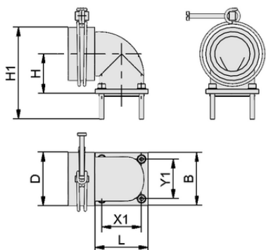
Design data SCHL-AN W 32.5-47x47x35 PSSG
