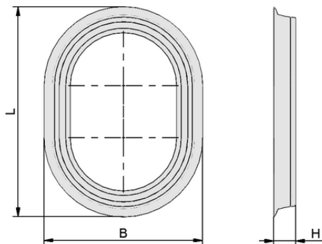
Design data DR-PSSG 290x215 NBR-60
