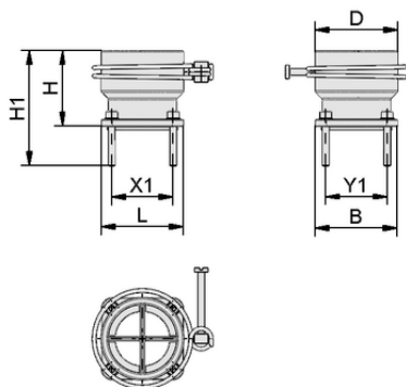
Design data SCHL-AN 32.5-47x47x48 PSSG
