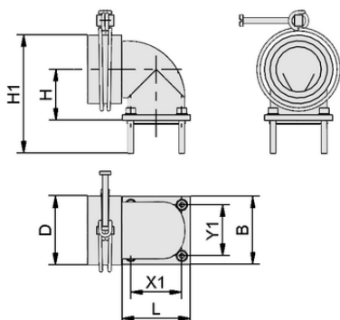
Design data SCHL-AN W 60.5-60x60x45 PSSG
