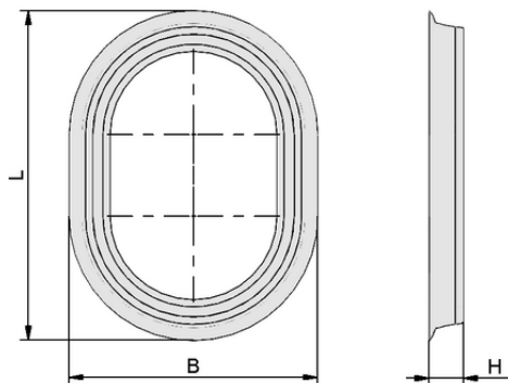
Design data DR-PSSG 405x305 NBR-60
