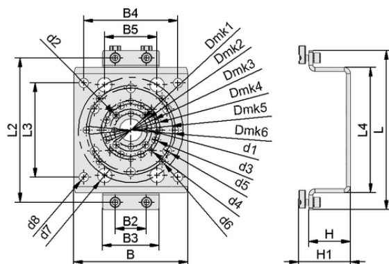
Design data MOD-FLAN 152x109 FXP/FMP-60
