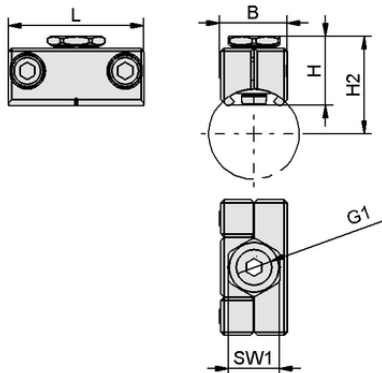
Design data SAUG-ANB G1/4-IG 42
