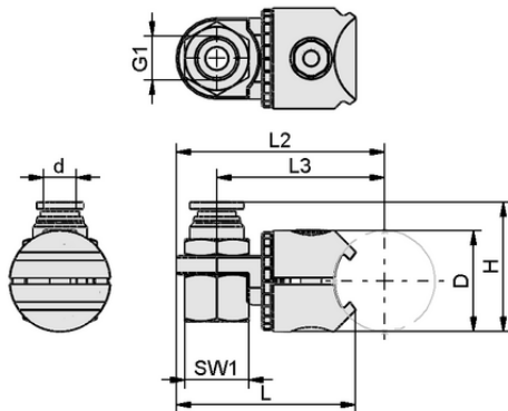
Design data SAUG-ANB PXT D30-I ROT
