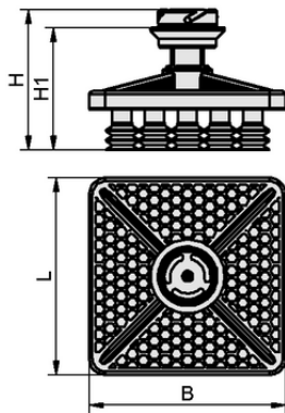
Design data RFBP 100 58 SPB2
