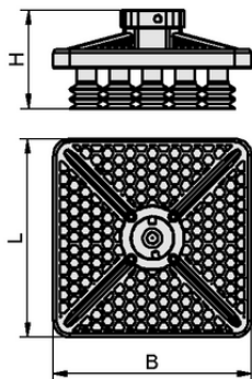
Design data RFBP 120 120 BA SPB2
