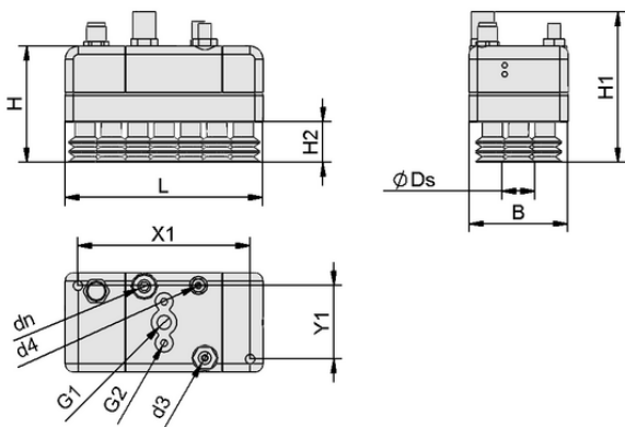
Design data FQE Xc 120x60 SW80 SPB2
