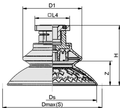
Design data SAXB 100 ED-85 RA
