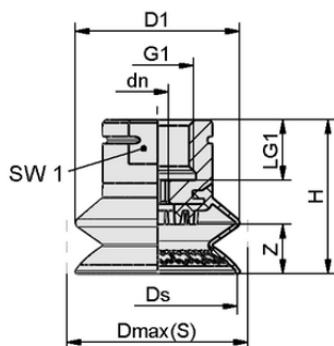
Design data SAXB 50 ED-85 G1/4-IG
