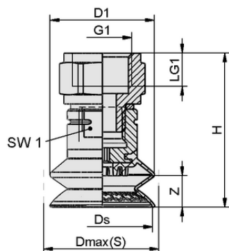
Design data SAXB 40 ED-85 G3/8-IG
