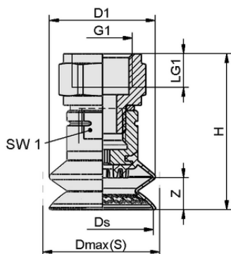
Design data SAXB 30 ED-85 NPT3/8-IG
