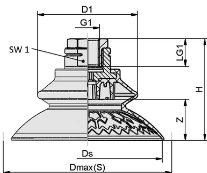
Design data SAXB 80 ED-85 NPT3/8-IG
