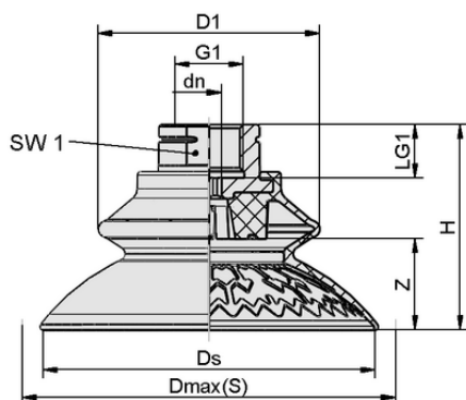
Design data SAXB 120 ED-85 G3/8-IG
