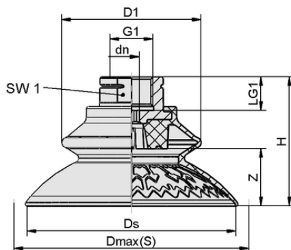
Design data SAXB 60 ED-85 G3/8-IG
