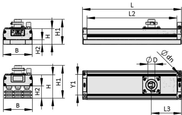
Design data FA-Mc SVK 1234 3R18 O20
