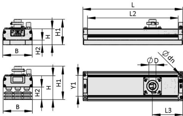
Design data FA-Mb SVK 442 3R54 SPB2-40P
