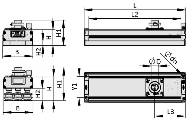
Design data FA-Mb SVK 442 3R18 O20
